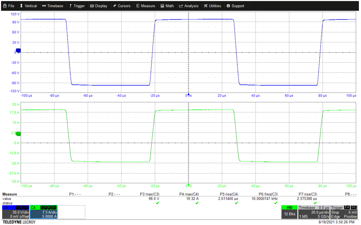
Figure 3: C3: Output Voltage; C4: Output Current V_{in} : 10 kHz, Load: 5 Ohm
