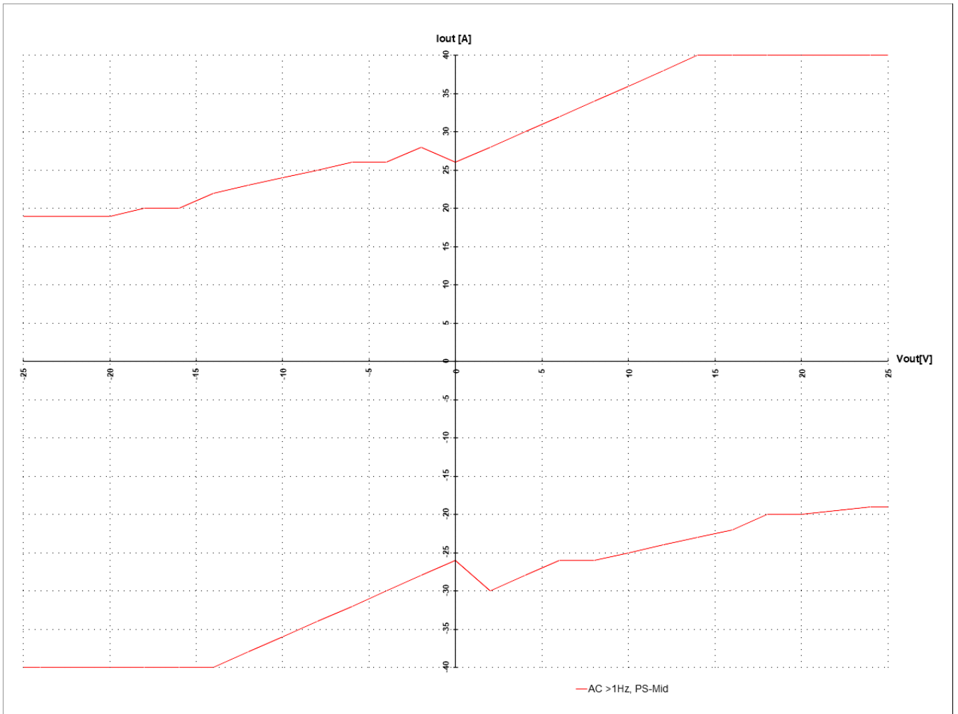
Figure 8: Operating Voltage: PS-Mid; Output Voltage: AC > 1 Hz
